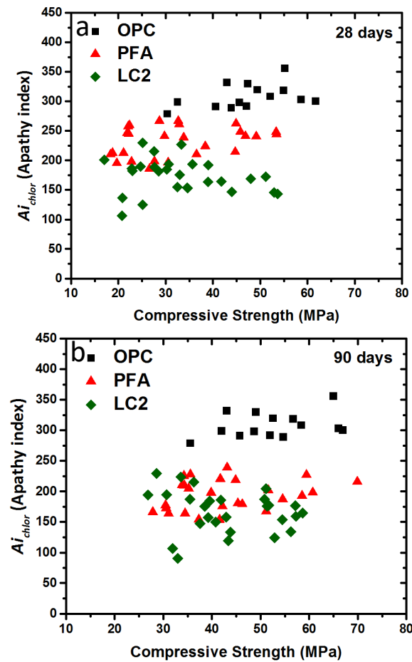
Figure 9. A-indices and compressive strengths of the different concrete systems.
