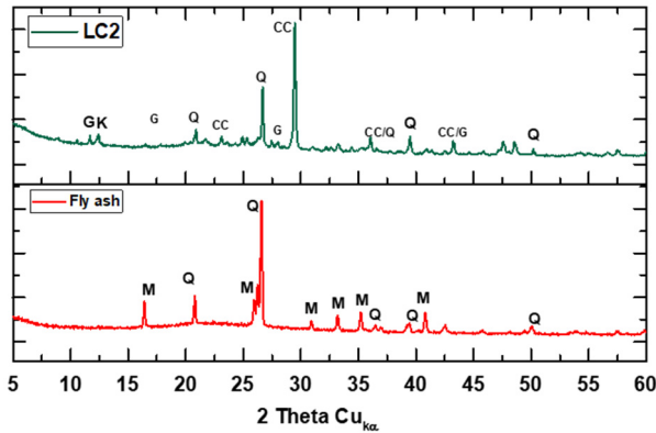
Figure 1. X-ray diffractogram of LC2 and fly ash used in the study. Reproduced with permission from Vaasudeva et al. [8].
