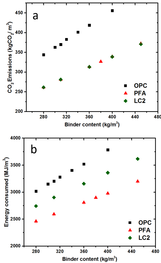
Figure 7. Energy and CO 2 emissions of different concretes used in the study.
