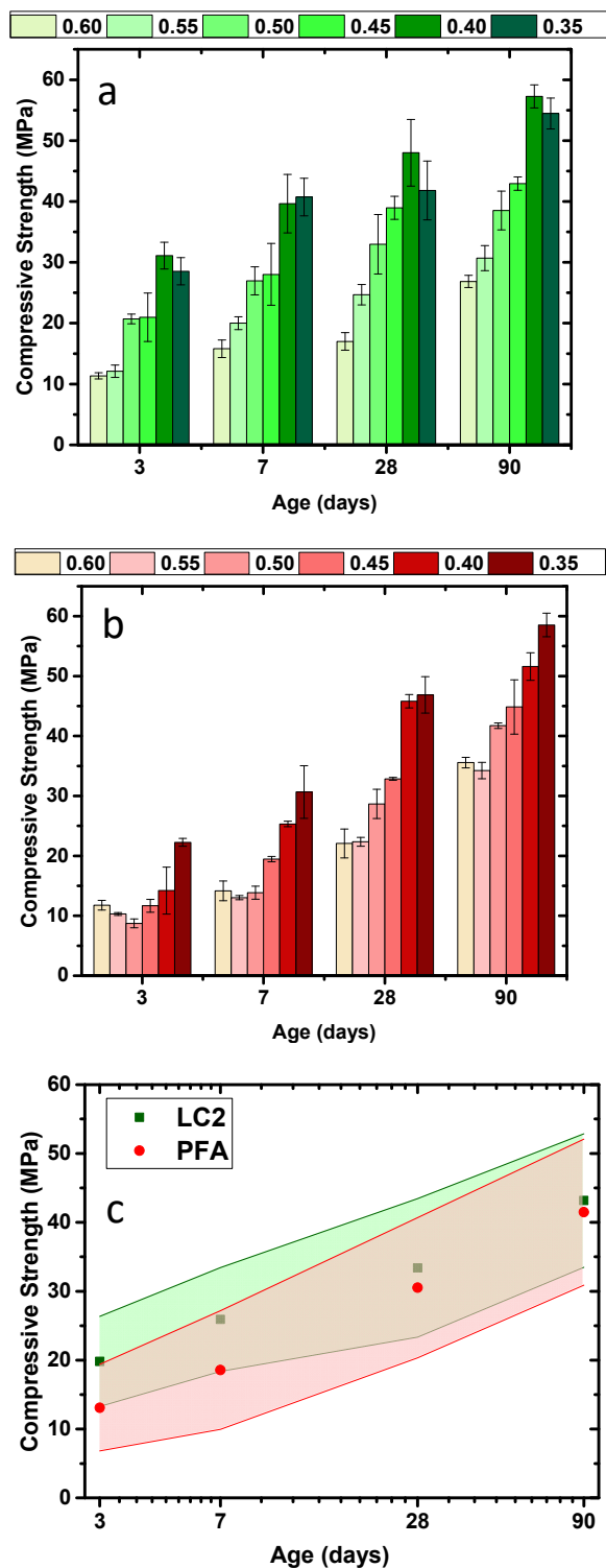
Figure 5. Strength development in concretes with binder content of 400 kg/m 3 having (a) LC2 with binder content of 400 kg/m 3 , and (b) PFA with binder content of 400 kg/m 3 ; and (c) strength development in all the concretes considered in the study
