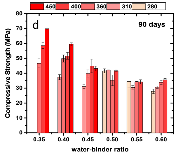
Figure 4. Compressive strength of concretes at 3 and 90 days: (a) LC2 at 3 days, (b) PFA at 3 days, (c) LC2 at 90 days, (d) PFA at 90 days.
