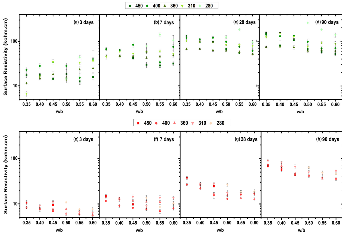
Figure 6. Surface resistivity of concretes with LC2 and PFA.
