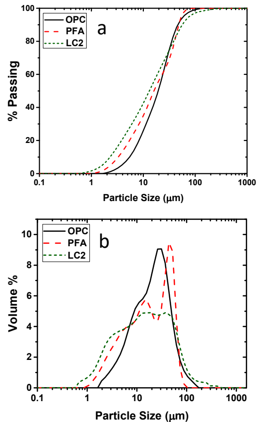
Figure 2. Particle size distributions of PFA, LC2 and OPC used in the study.
