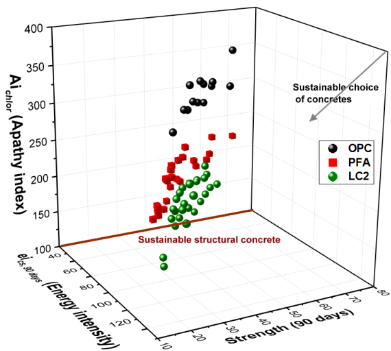
Figure 11. Sustainability framework with the dependence on concrete strength.
