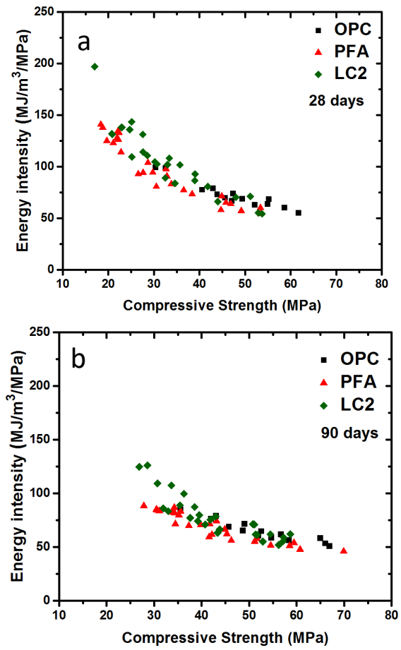
Figure 8. Variation of energy intensity indices with compressive strength, for different binders.
