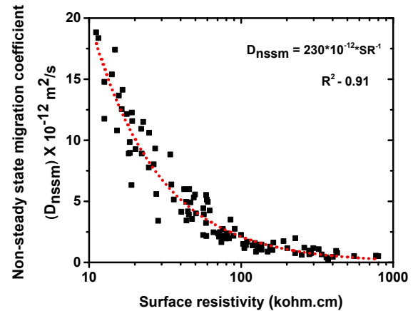
Figure 3. Relationship between surface resistivity (SR) and non-steady state migration coefficient based on previous studies at IIT Madras.
