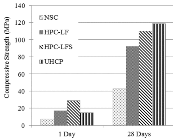
Fig. 11 Compressive strength of concrete at 1 day and 28 days.
