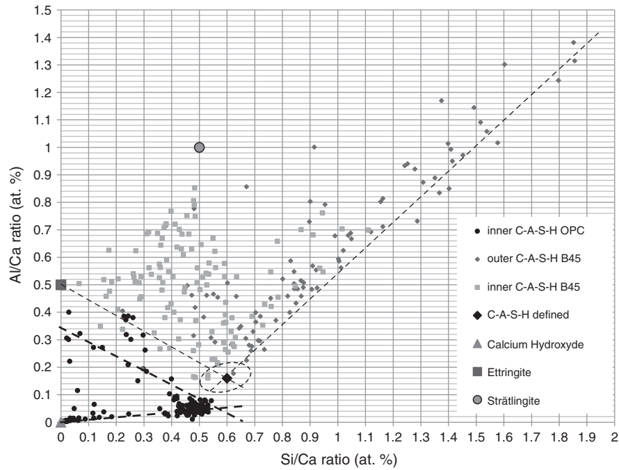
Fig. 8. Graphical treatment of EDS points analysis obtained on a B45 300 d old paste, Al/Ca ratio is plotted as a function of Si/Ca ratio (in atomic percentage). X-ray volume of interaction at the used acceleration voltage (15 kV) is about 1 \mu\text{m} , resulting in intermixing of C–A–S–H with ettringite, strätlingite and non-reacted metakaolin. The dotted lines join C–A–S–H with ettringite and with ettringite and form the lower limits in term of Al/Ca ratio of the cloud of measured points. The C–A–S–H composition in the blend lies within the dotted circle but cannot be precisely defined. The chosen C–A–S–H composition for mass balance calculations is represented. For comparison inner C–A–S–H of OPC is given, where intermixing with portlandite and AFm/AFt is observable.
