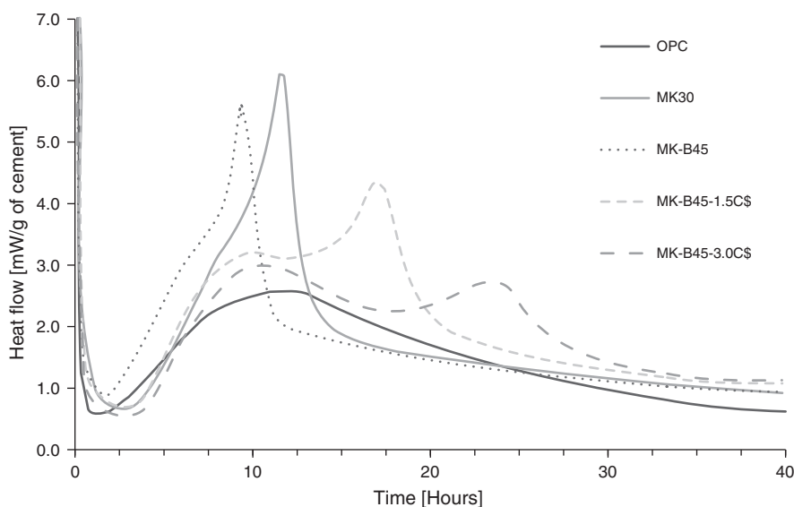
Fig. 13. Isothermal calorimetric curves plotted for blend systems at 45% substitution with different gypsum contents.
