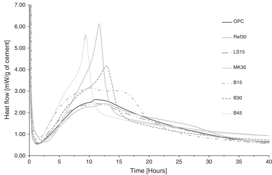
Fig. 11. Isothermal calorimetry curves of the blend pastes (water/binder ratio 0.4) until 40 h. The higher the cement replacement by the blend, the higher the secondary aluminates peak.
