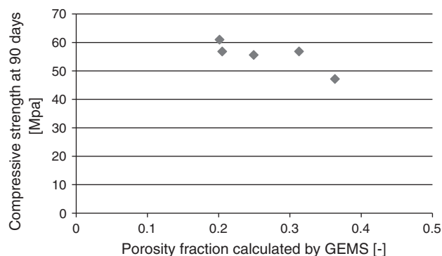
Fig. 15. Compressive strength at 90 days represented as a function of its corresponding porosity calculated by GEMS.
