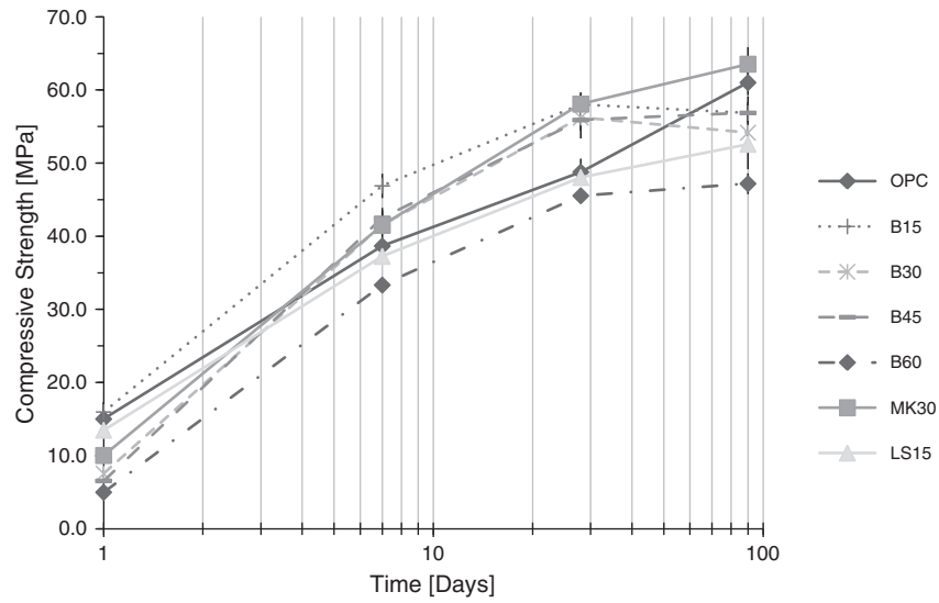
Fig. 2. Compressive strength of blends mortars at 1, 7, 28 and 90 days.
