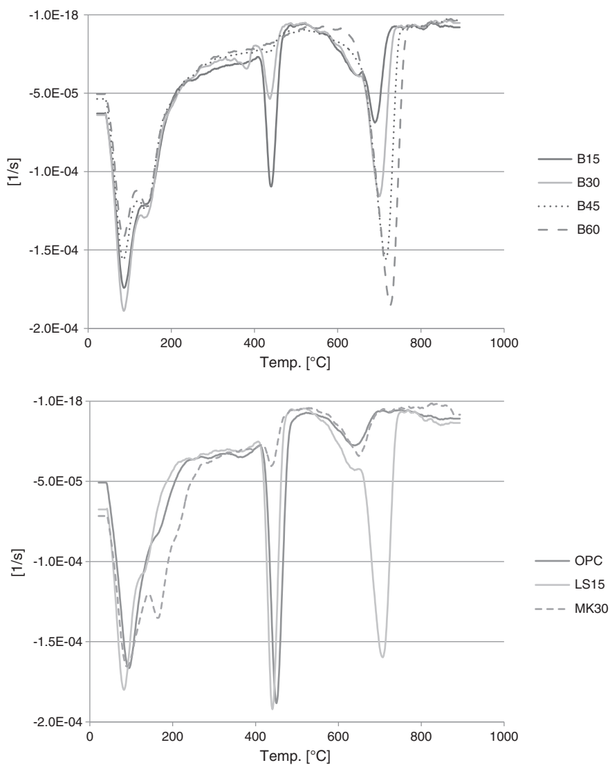
Fig. 5. Time derivative of the mass loss as a function of the increasing temperature obtained by TGA analysis of samples at 90 days.
