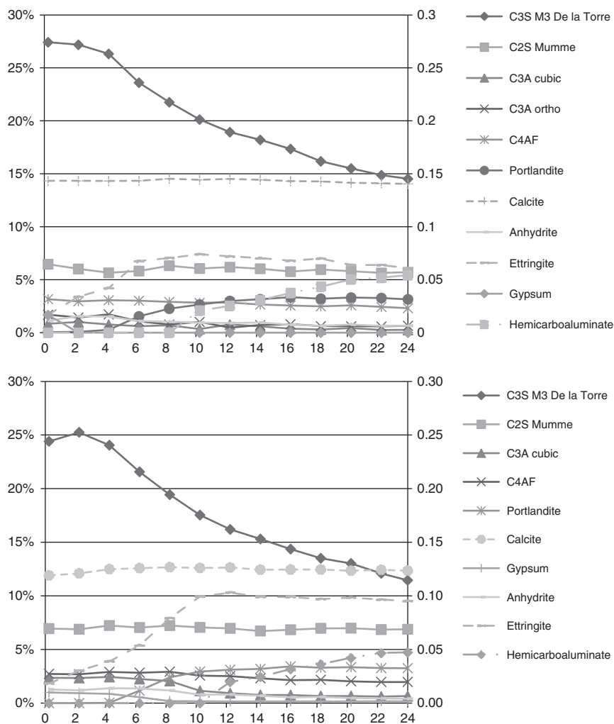
Fig. 14. Evolution of phases obtained by Rietveld refinement of in-situ XRD during the first 24 h of hydration for B45 (top) and B45 + 1.5 wt.% gypsum (bottom). Gypsum addition enhances C_3S hydration as well as ettringite formation.
