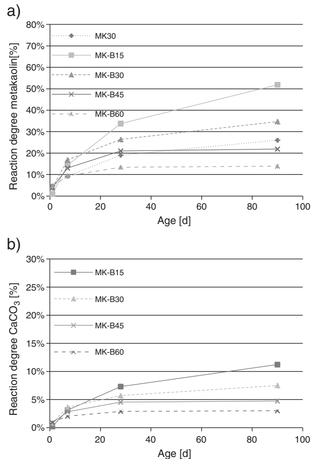
Fig. 9. Metakaolin (a) and limestone (b) reactivities calculated by mass balance.
