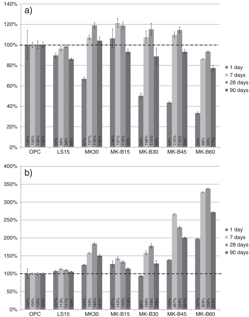
Fig. 3. a) and b): Compressive strength of blends normalized to the strength of pure PC (a) and to the quartz reference (b) mortars at 1, 7, 28 and 90 days.
