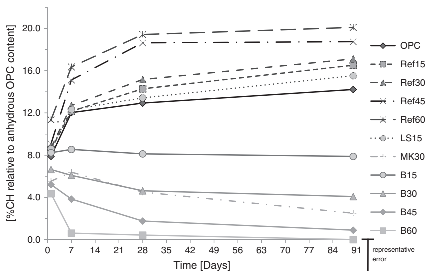
Fig. 4. Evolution of the CH content (determined from TGA mass loss) normalized to the PC content in the paste.
