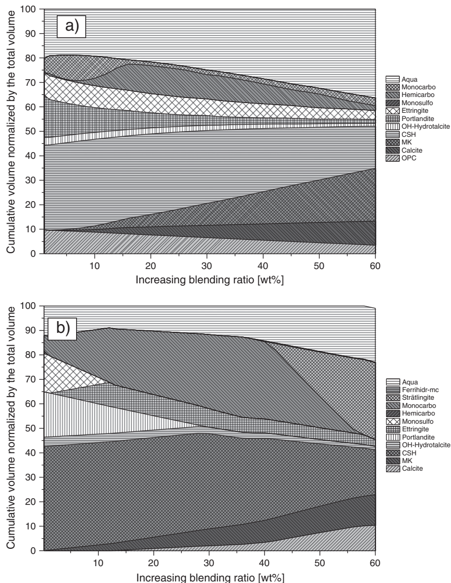
Fig. 10. a) and b): Thermodynamic simulations of the phase assemblage with increasing substitution of cement by our 2:1 metakaolin:limestone blend. The total cumulative volume of solid products is represented as a function of increasing percentage. In the first figure the reactivities of limestone and metakaolin obtained from mass balance calculations in the hypothesis of formation of hemicarboaluminate and real C_{1.67}A_{0.27}SH_x are used, while in the second the limestone is let freely reacting and metakaolin fixed at 50% reactivity. PC was supposed to react at 80% in case a) and 100% in case b).
