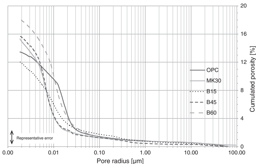
Fig. 7. Cumulated porosity as a function of pore entry radius at 28 days obtained by mercury intrusion porosimetry.
