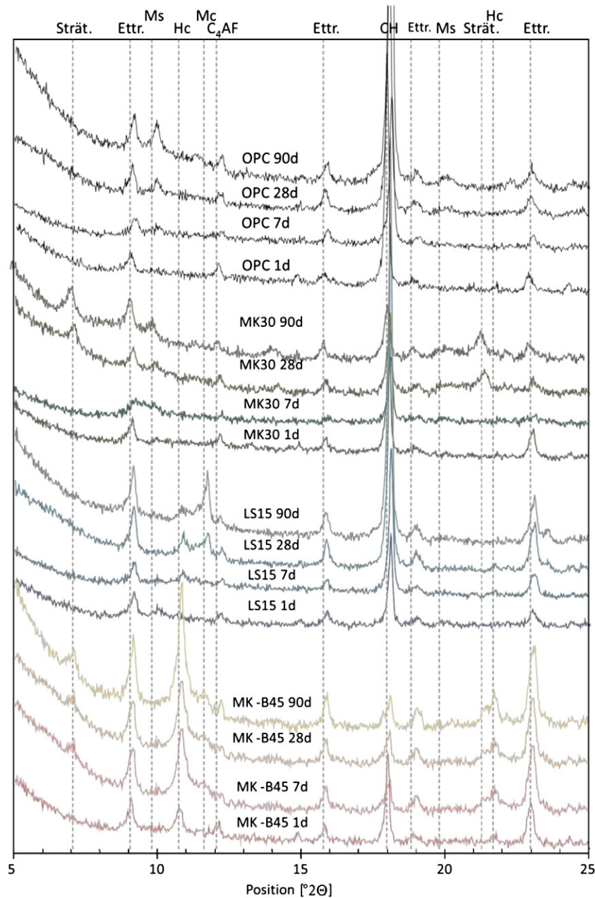
Fig. 6. XRD patterns for PC, MK30, LS15, and MK-B45 at 1, 7, 28 and 90 days. While in PC ettringite and monosulfoaluminate (Ms) hydrate form, MK addition leads to the formation of strätlingite (Strät) and reduction of the portlandite peak (CH). With limestone addition in both LS15 and blend systems, formation of hemicarboaluminate (Hc) and later on monocarboaluminate (Mc) are observed.
