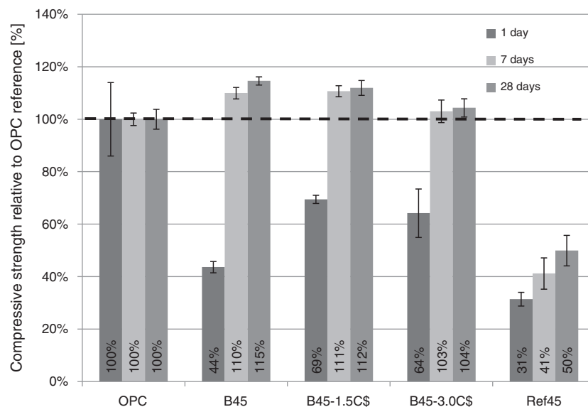
Fig. 12. Evolution of the mechanical strength of blend systems at 45% substitution as a function of the gypsum added at all ages.
